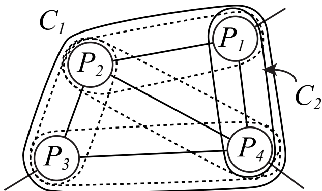
Fig. 2 Illustration of the selection of negative examples from complexes with size more than two.
