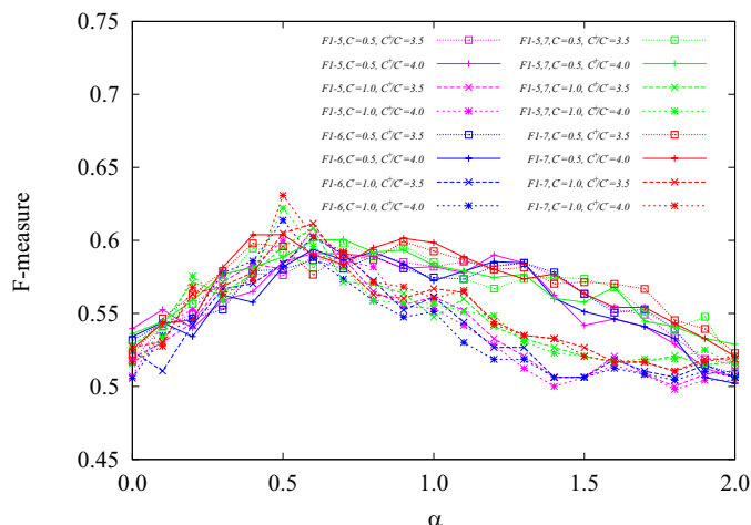
Fig. 3 Result on the average F-measures using four sets of features and the domain composition kernel with \alpha = 0.0, 0.1 \dots, 2.0 .
