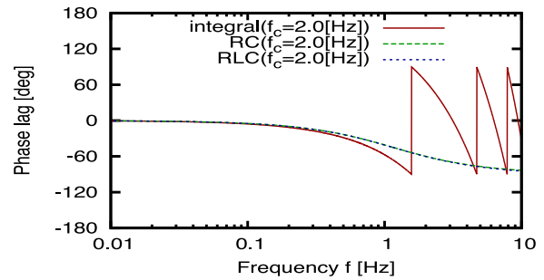
Fig. 5 Phase lags of the integral filter, the RC filter, and the RLC filter for the cutoff frequency f_c = 2.0 [Hz].
