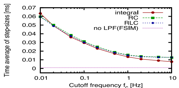
Fig. 15 Average step-size of the integral filter, the RC filter, and the RLC filter for different cutoff frequencies f_c when using the simple scenario.
