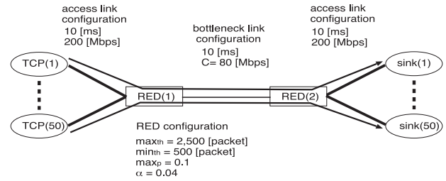
Fig. 7 Dumbbell topology.
