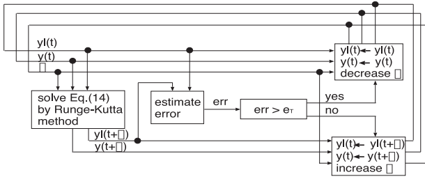
Fig. 6 Block figure of network updates.
