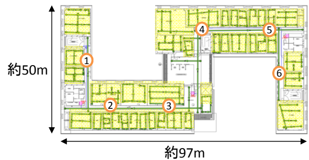
図 4 既設無線 LAN Fig. 4 Existing WLAN infrastructure
