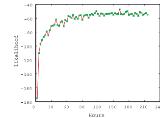
Fig. 9 Learning curve.
