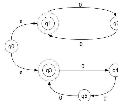
図 3 Non-deterministic Finite Automaton
