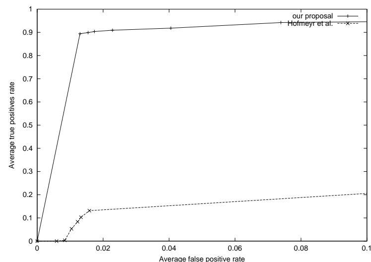
図 8 named に関するデータを用いた異常検知の結果 (ROC 曲線) ( N = 6, D = 5 ) Fig. 8 The experimental result (ROC curve) using named data set ( N = 6, D = 5 )
