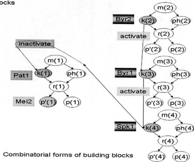
Figure 6 Interaction between the signaling cascade of MAP kinases and the Pat1-Mei2 pathway
