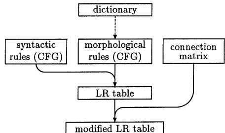
Fig. 8 Outline of generating a modified LR table
