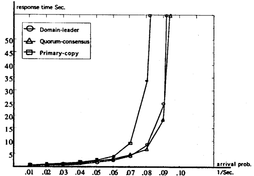
fig.10: write request response time when arrival probability is 80%(10 replicas).
