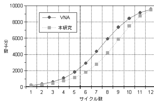
図 6 両シミュレータにおける" Tem "分子の数の変化 Fig. 6 Changes of " Tem " molecules in both simulator
