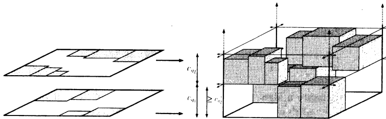
Figure 7: Layer packing of S_{small}
