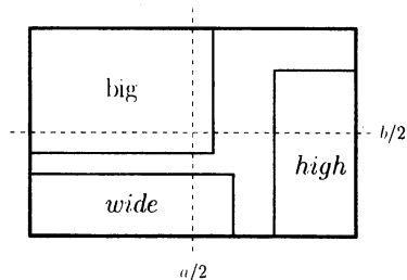
Figure 1: Wide, high and big items
