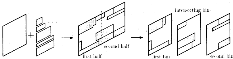
Figure 5: Packing the projections of S_a into three bins
