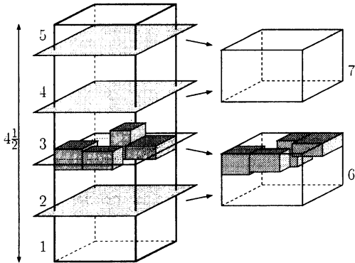
Figure 8: Layer packing of S_{small}
