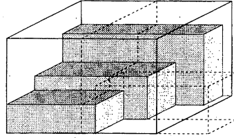
Figure 2: Packing of long items in direction a
