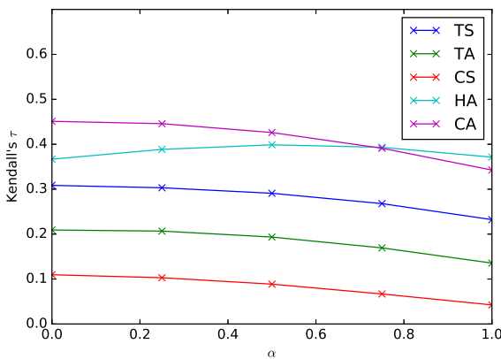
Fig. 5 Effect of \alpha on the \tau between average subjective ratings and AUCH.
