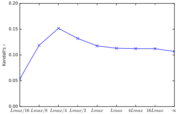
Fig. 4 Effect of L on the \tau between average customer satisfaction and AUCH.
