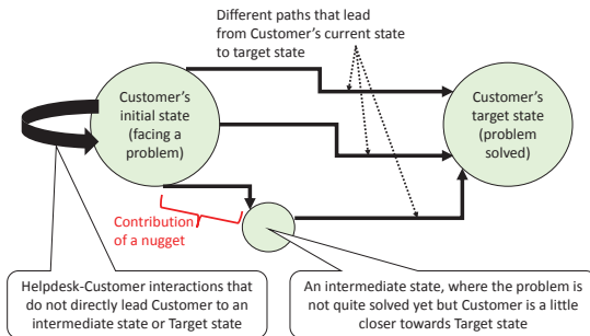
Fig. 3 Task accomplishment as state transitions, and the role of a nugget.
