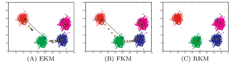
Fig. 10 Clustering results when an undefined cluster exists.
