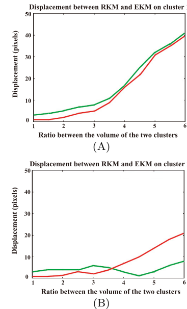
Fig. 14 The displacements between the EKM and RKM on each cluster in the case of Fig. 13. Green curve: the displacement of RKM; Red Curve: the displacement of EKM
