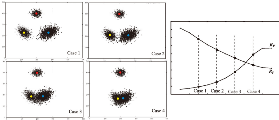
Fig. 7 Investigation on the possibility of merging two clusters.
