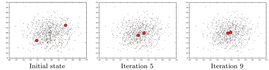
Fig. 6 In one crowd of data vectors, RK-means will merge two initial cluster centers together.
