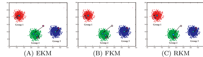
Fig. 11 Clustering results when a redundant cluster exists.
