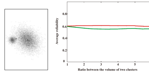
Fig. 13 Experiment of the RK-means clustering under variable distribution. In the right graph, the horizontal axis shows the ratio between the volumes of two clusters, the vertical axis shows the average reliability of each cluster. The red curve shows the average reliability of the left cluster, and the green one shows that of the right cluster.
