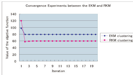
Fig. 12 Convergence of the EKM and the RKM algorithms.
