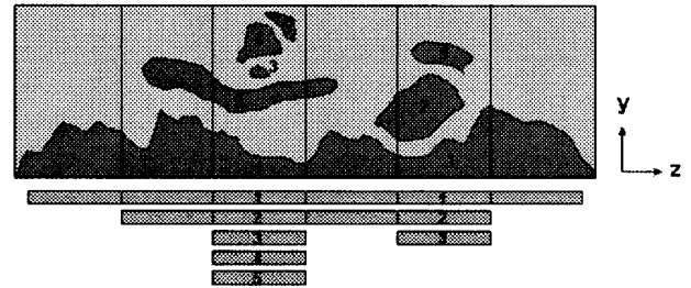
Fig.4. Memory management: The scene is stored in textures, where each texture can store one y-layer. The textures are indicated as grey blocks below the scene
