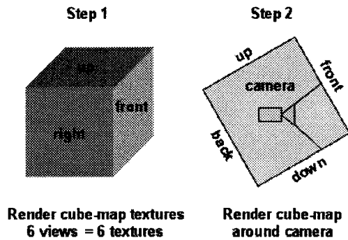
Fig.2. 6 DOF by using a cube-map: The scene is rendered in six directions in a first step, where each direction is equal to one texture on the cube-map. In the second step, the cube-map is rendered around the camera.
