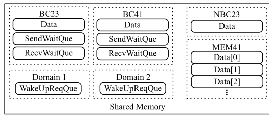
Fig. 4 The data structure of shared memory.
