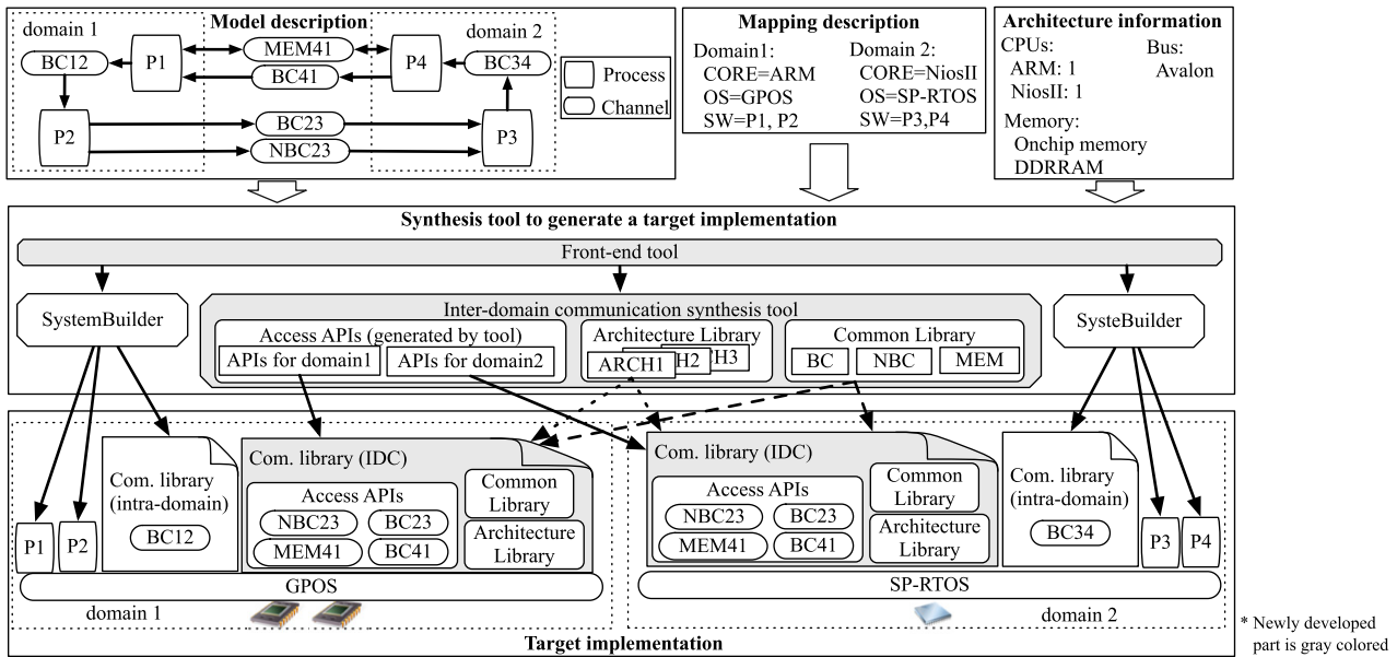
Fig. 2 An automatic communication synthesis tool and an example of target implementation.
