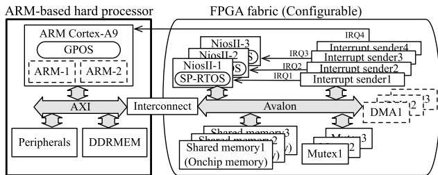
Fig. 1 An example of a Hetero-MP on Altera SoC.
