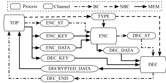
Fig. 5 Model description of AES encryption and decryption application.
