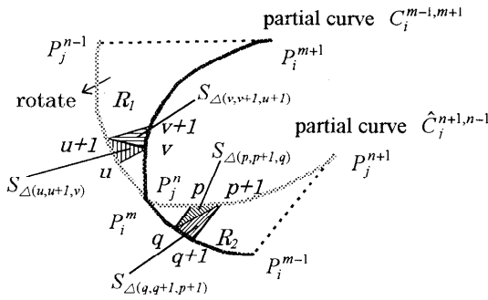
Fig. 4 Partial curve \hat{C}_j^{n+1, n-1} is translated so that the dominant point P_j^n and the dominant point P_i^m overlap, and is then rotated clockwise.
