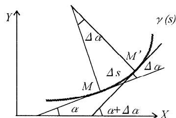
Fig. 2 Intrinsic definition of curvature.
