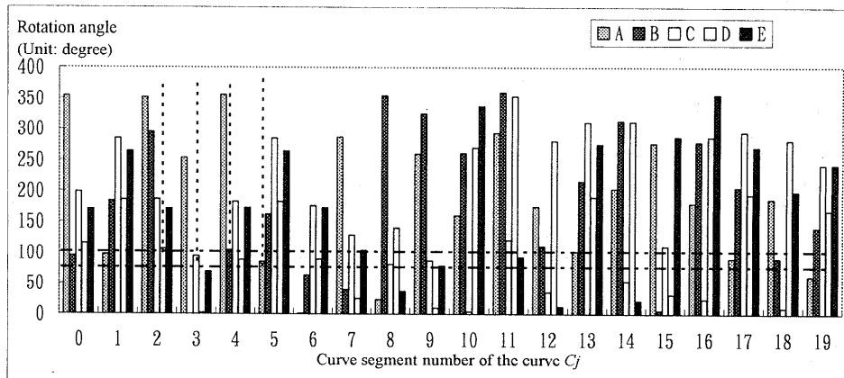
Fig. 17 Rotation angles of all curve segments of the object on left when it is matched with curve segments 17-19, 0-1 (shown by A-E) of the object on the right in Fig. 5.
