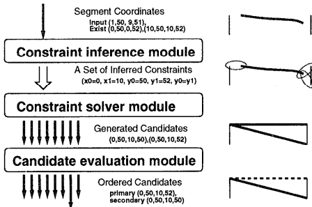
図9 整形処理部の処理の流れ Fig. 9 Structure of the beautification routine.
