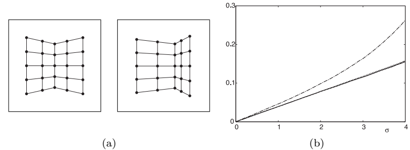
Fig. 2 (a) Simulated images of planar grid surfaces. (b) The RMS error vs. noise level \sigma . The plot for our algorithm (solid line) and plot for the alternative method (dashed line) completely overlap. Chained line: the 8-point algorithm. Dotted line: KCR lower bound.
