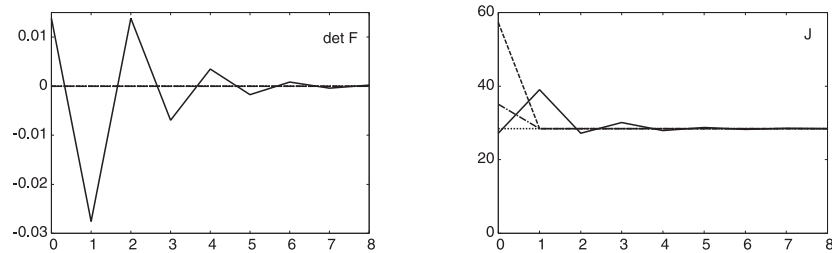
Fig. 4 The corresponding results by EFNS.
