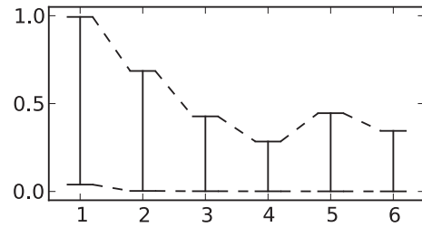
Fig. 3 Upper and lower bounds of relative weight of harmonic partials of reference signals.
