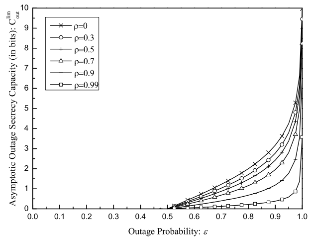
Fig. 6 The asymptotic outage secrecy capacity versus outage probability, for some selected values of channel power correlation coefficients (PCC) and for the channel scenario of \kappa = 0 dB.
