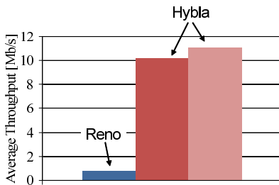
Fig. 6 Average throughputs of TCP flows: Different kinds of TCPs (Reno x 1 + Hybla x 2).
