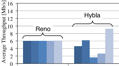
Fig. 5 Average throughputs of TCP flows: One kind of TCP (five flows).
