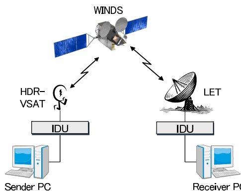
Fig. 1 Experimental environment for performance comparison.
