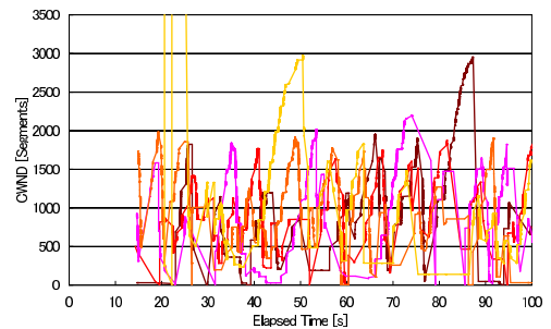
Fig. 10 CWND of each TCP flow: Hybla x 5.
