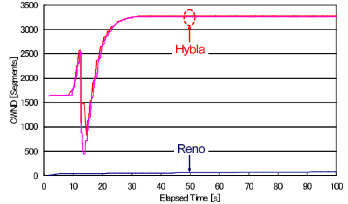
Fig. 8 CWND of each TCP flow: Reno x 1 + Hybla x 2.
