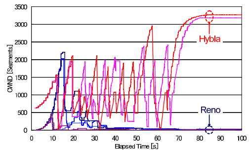
Fig. 9 CWND of each TCP flow: Reno x 5 + Hybla x 2.
