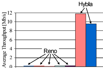
Fig. 7 Average throughputs of TCP flows: Different kinds of TCPs (Reno x 5 + Hybla x 2).
