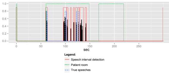
Fig. 4 Result of integrated process. After detecting patient rooms (green-dotted line) by walking detection and location estimation, we apply speech interval estimation (black line which is smoothed to the red-solid line). Compared with the ground truth of the speech sentences of nurses (blue-dashed line), it covers all of the ground truth regions.
