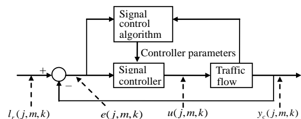
Figure 3 Signal control system of congestion length at each signalized intersection.
