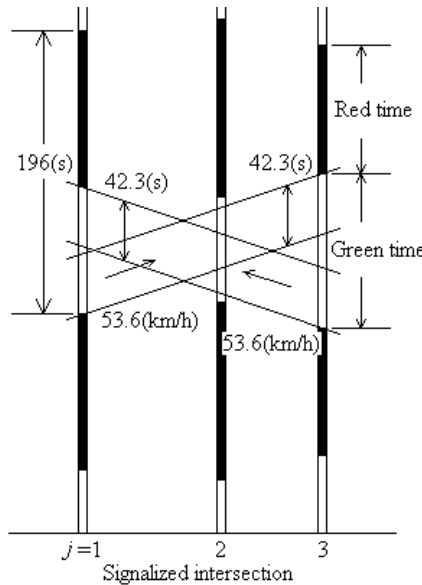
Figure 11 Balance offset for straightforward vehicles at three signalized intersections.
