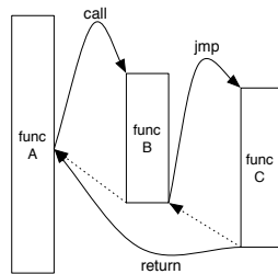
図 9 Tail Call Elimination
