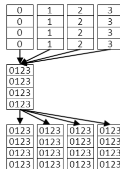
図 1 Reduce + Bcast
