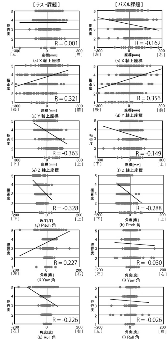
図3 頭部位置・姿勢と割り込み拒否度の関係 Fig. 3 Relationship between head position and unavailability.
