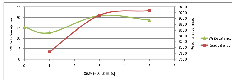
(b) Latency
