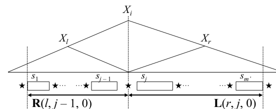
Fig. 4 Illustration of Algorithm 2. If k = 0 , \mathbf{R}(\ell, j - 1, 0) \neq \infty and \mathbf{L}(r, j, 0) \neq \infty , then (|X_\ell| - \mathbf{R}(\ell, j - 1, 0), |X_\ell| + \mathbf{L}(r, j, 0) - 1) is a candidate of a crossing occurrence.
