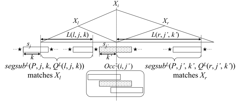
Fig. 2 Illustration of Equation (4) of Lemma 7. j' and k' can be computed in O(1) time. Then, Q^L(i, j, k) and L(i, j, k) can be also computed in O(1) time. Since s_{j'} and s_{j'-1} cannot overlap, k' must satisfy k' + L(l, j, k) \leq |X_\ell| .
