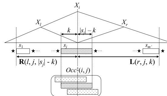
Fig. 3 Illustration of Algorithm 2. If k \in \text{Occ}^\dagger(X_i, s_j) , \mathbf{R}(\ell, j, |s_j| - k) \neq \infty and \mathbf{L}(r, j, k) \neq \infty , then (|X_\ell| - \mathbf{R}(\ell, j, |s_j| - k), |X_\ell| + \mathbf{L}(r, j, k) - 1) is a candidate of a crossing occurrence.
