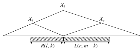
Fig. 1 If R(\ell, k) \neq \infty and L(r, m - k) \neq \infty , there is a crossing subsequence occurrence of P . P[0 : k - 1] is a subsequence of X_\ell[|X_\ell| - R(\ell, k) : |X_\ell| - 1] , and P[k : m - 1] is a subsequence of X_r[0 : L(r, m - k) + 1] .
