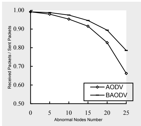
Figure 3 Impact of Packet Delivery Ratio by Nodes Abnormal Comparison
