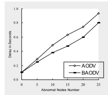
Figure 5 Impact of Routing Delay by Nodes Abnormal Comparison
