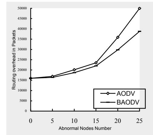
Figure 4 Impact of Routing Overhead by Nodes Abnormal Comparison
