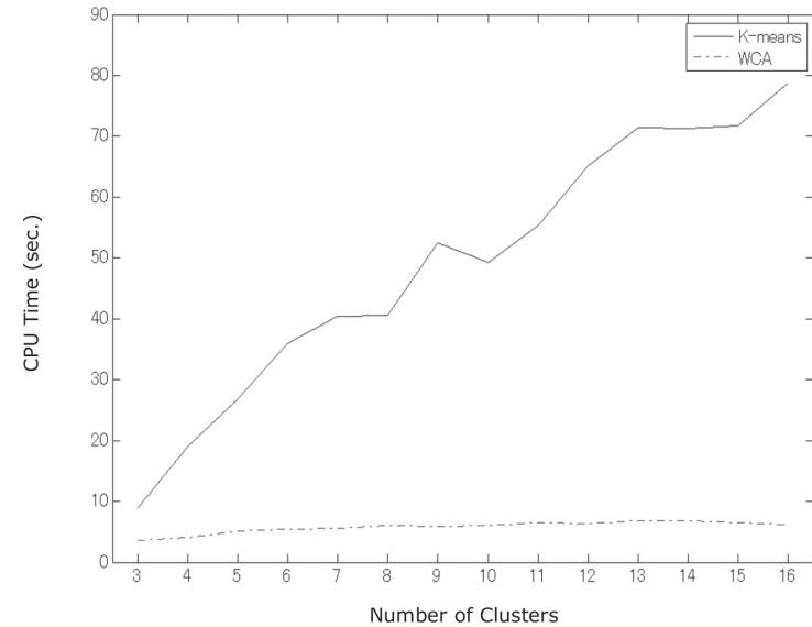
Fig. 7 CPU time of CLASSIC3.
