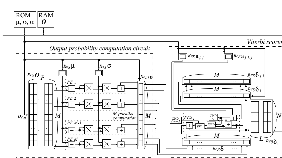
Fig. 7 FastStoreBPP VLSI architecture ( [M/P] = 1 ).
