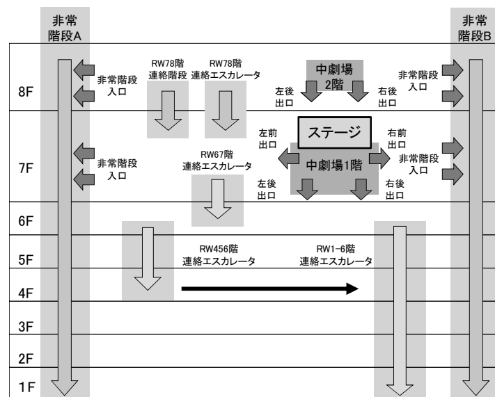
図4 北九州芸術劇場中劇場（リバーウォーク北九州 7,8階）から1階までの避難経路 Fig. 4 Evacuation route from 7th and 8th floor (Kitakyushu Performing Arts Center) to 1st floor of RIVERWALK KITAKYUSHU
