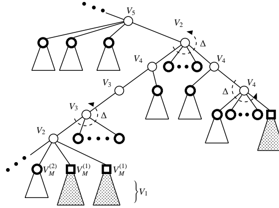
Fig.1 Partition of V into V_i 's ( i = 1, \dots, 5 ). Bold circles are leaves ( V_L ) or pseudo-leaves ( V_M^{(2)} - V_L ) with their subtrees, while bold squares are vertices in V_M^{(1)} with their subtrees.
