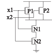
Fig. 1 two-input NAND gate.
