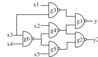
Fig. 3 c17 benchmark circuit.
