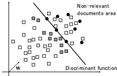
Fig. 4 Mapped non-checked documents into the feature space: Boxes denote non-checked documents which are mapped into the feature space. Circles denotes checked documents which are mapped into the feature space. Gray boxes denotes the displayed documents to a user in the next iteration. These documents are in the “not non-relevant document area” and near the discriminant hyperplane.
