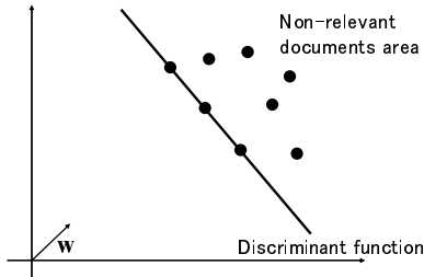
Fig. 3 Generation of a hyperplane to discriminate non-relevant documents area: Circles denote documents which are checked non-relevant by a user. The solid line denotes the discriminant hyperplane.
