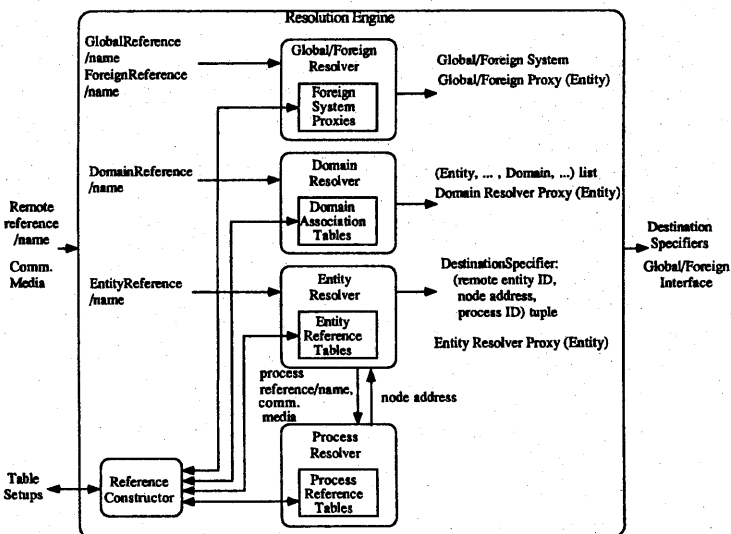
図 3. Reference Resolution and Resolution Engine
