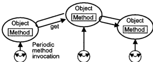
(b) Time-Triggered Object Model
