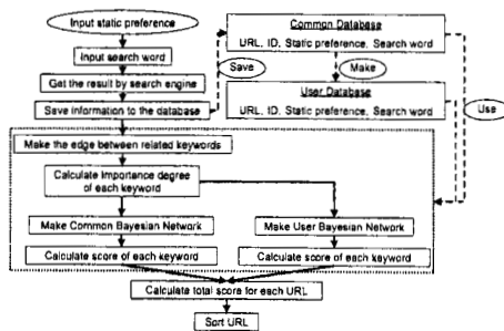
Fig. 1: Web Search Filtering Algorithm
