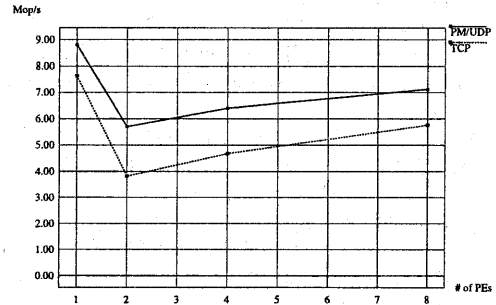
図 10 NPB2.3: IS (Class S)
