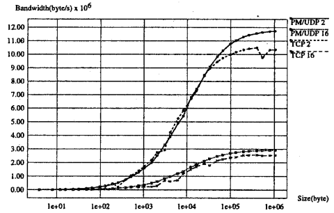
図5 MPI: Broadcast
