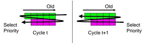
図9 RR(Round-Robin) 調停
