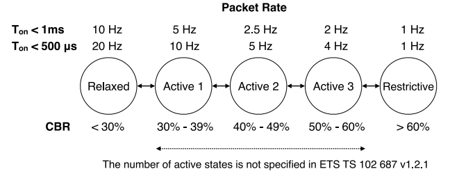
Fig. 2 ETSI DCC reactive algorithm.
