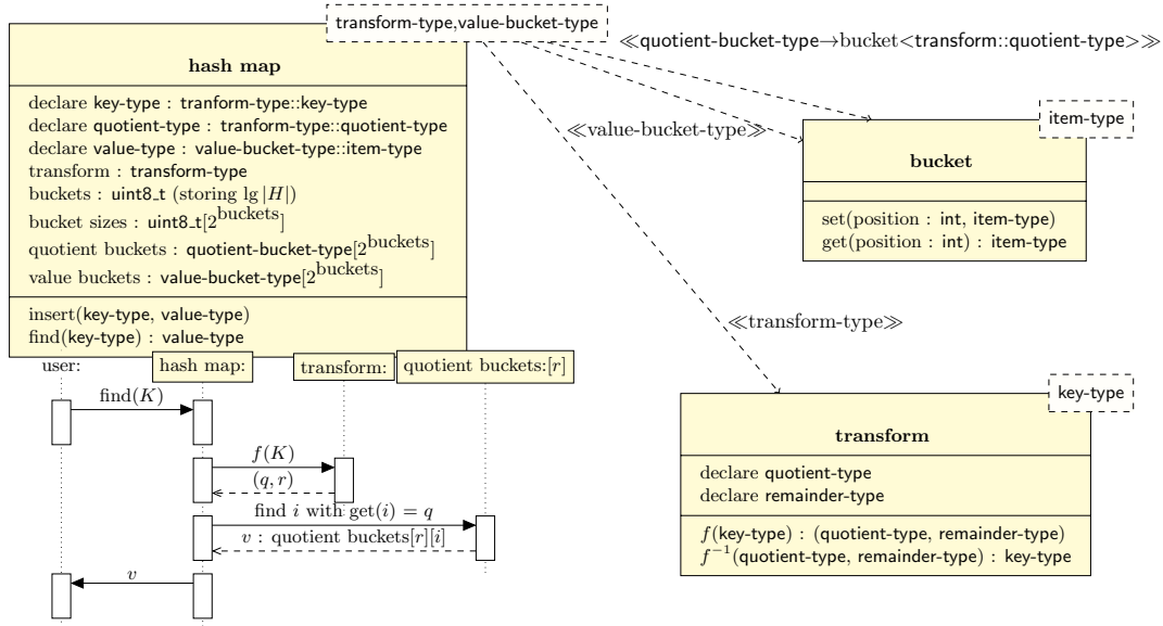
Fig. 1 Diagram of our proposed hash table. The call of \text{find}(K) returns the i -th element of the r -th bucket at which K is located. The injective transform determines the types of the key and the quotient.
