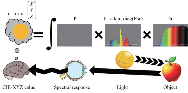
図 1 Mechanism of perception of visible light
