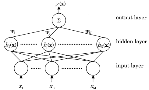
Fig. 6 Structure of an RBF network.
