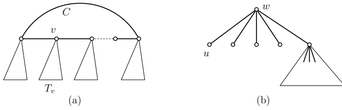
Fig. 1 (a) The tree T_v corresponding to v \in V(C) . (b) A safe degree-1 vertex u of a tree.
