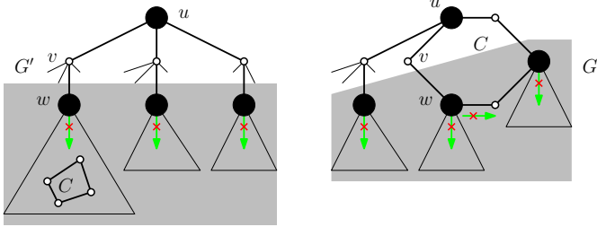
Fig. 2 Case (i) of Lemma 3.1. The token on u is (G, \mathbf{I}) -rigid.
