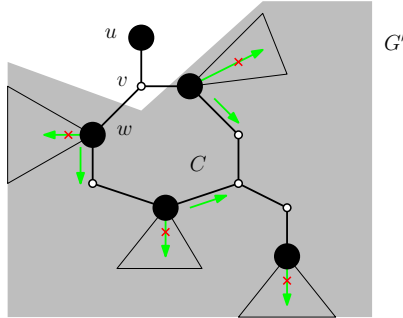
Fig. 3 Case (ii) of Lemma 3.1. The token on u is (G, \mathbf{I}) -rigid.
