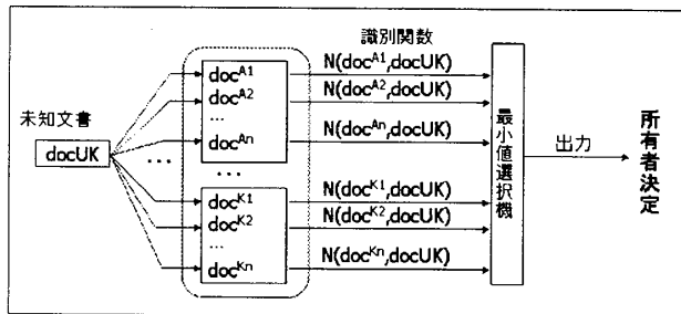
図 2: Nearest Neighbor Rule.
