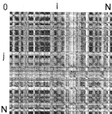
図2 Distance Matrix
