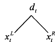
図1: Joint Stereo
