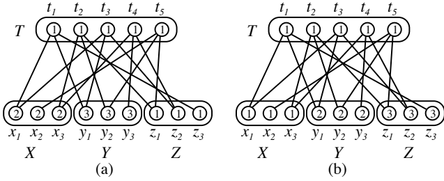
Fig. 2 (a) The initial token-placement and (b) the target token-placement of the graph constructed from an instance (X = \{x_1, x_2, x_3\}, Y = \{y_1, y_2, y_3\}, Z = \{z_1, z_2, z_3\}, T = \{t_1 = (x_1, y_1, z_3), t_2 = (x_3, y_2, z_1), t_3 = (x_1, y_1, z_2), t_4 = (x_3, y_3, z_2), t_5 = (x_2, y_2, z_1)\}) .
