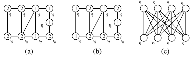
Fig. 4 (a) An initial token-placement. (b) The target token-placement. (c) The weighted complete bipartite graph constructed from (a) and (b) (the weight of each edge is omitted).
