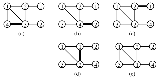
Fig. 1 An example of 4-COLORED TOKEN SWAPPING. Tokens of vertices are written inside circles. We swap the two tokens along each thick edge. (a) An initial token-placement. (b)–(d) Intermediate token-placements. (e) The target token-placement.
