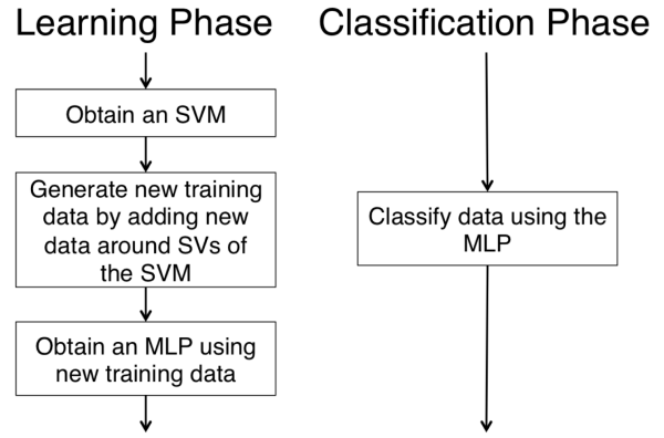
Fig. 3 Brief flows of the DBM algorithm. There are 3 steps in the learning phase, and 1 step for classification step.
