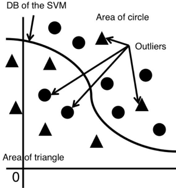
Fig. 4 An example of SVM-based outlier detection. An outlier lies on the wrong side of its own area.
