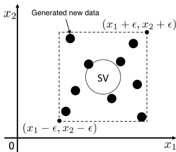
Fig. 1 New data is generated in \epsilon -neighborhood area of the SV.
