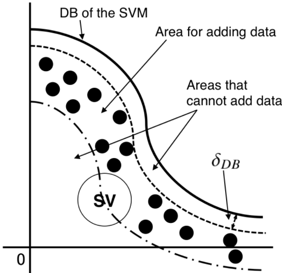
Fig. 2 Two conditions of the DBM algorithm are shown in this figure. DBM does not add new data in [-\delta_{DB}, \delta_{DB}] and farther area than that of SVM.
