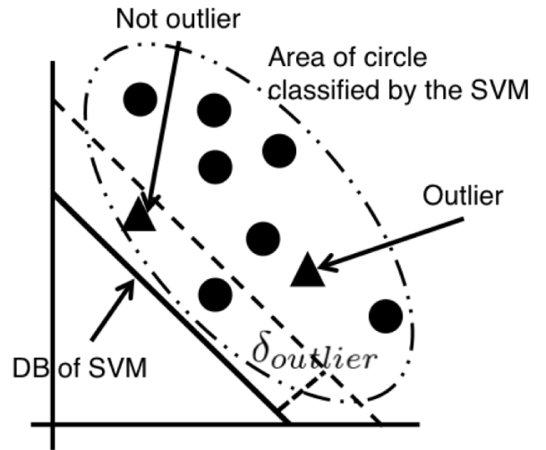
Fig. 5 \delta_{outlier} defines the range of noisy data (outliers) that influence performance of machine learning models. Vectors within the range of \delta_{outlier} area are detected as outlier data.
